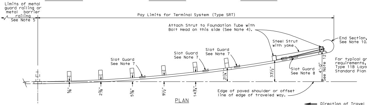
PLAN
