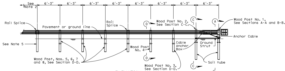
ELEVATION TERMINAL SYSTEM (TYPE SKT)
